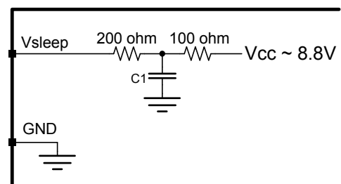
Figure 14: Vsleep output
