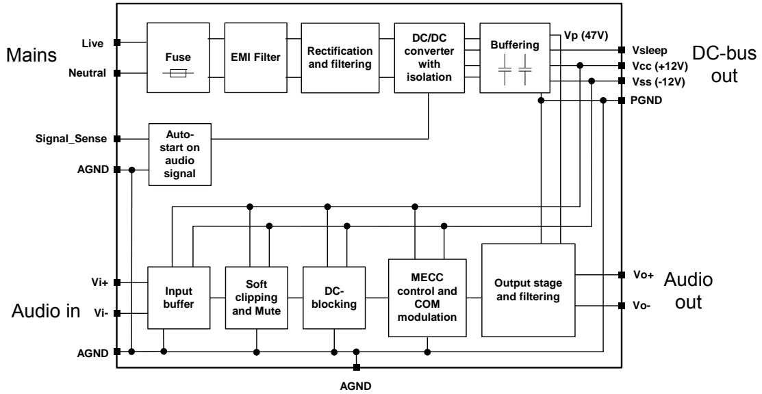
Figure 1: ICEpower200ASC block diagram
