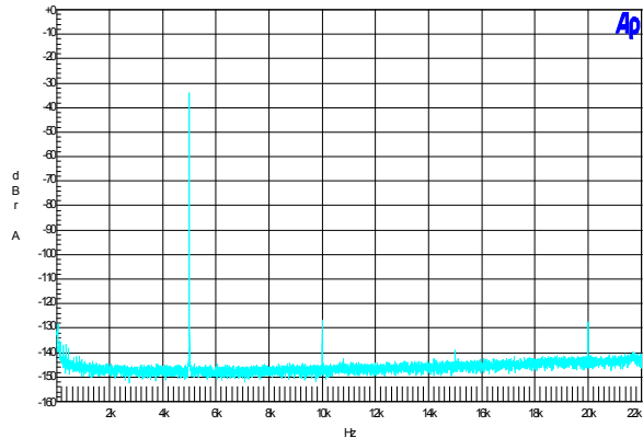
f = 5kHz. Po = 100mW. 4Ω loading.
