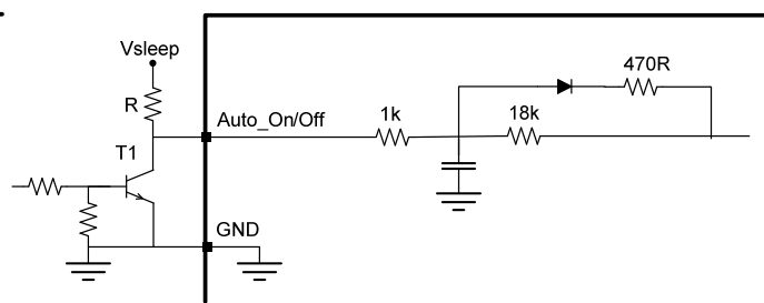
Figure 16: Controlled On/Off application
