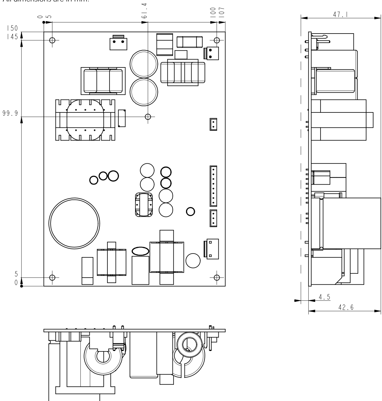
Figure 24: Physical dimensions in mm.
