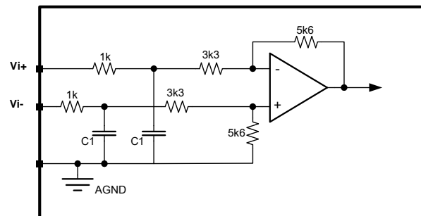
Figure 18: Balanced input buffer.
