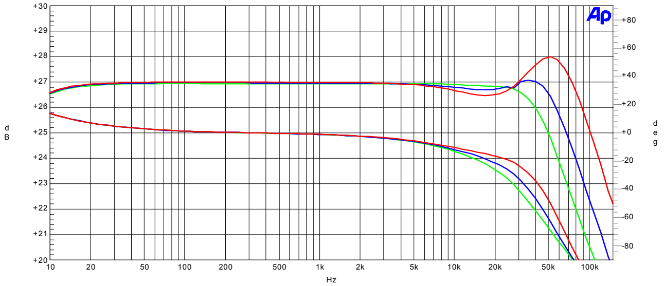
Figure 3: Frequency response in 4Ω (green), 8Ω (blue) and open load (red). Top – amplitude. Bottom – phase.
