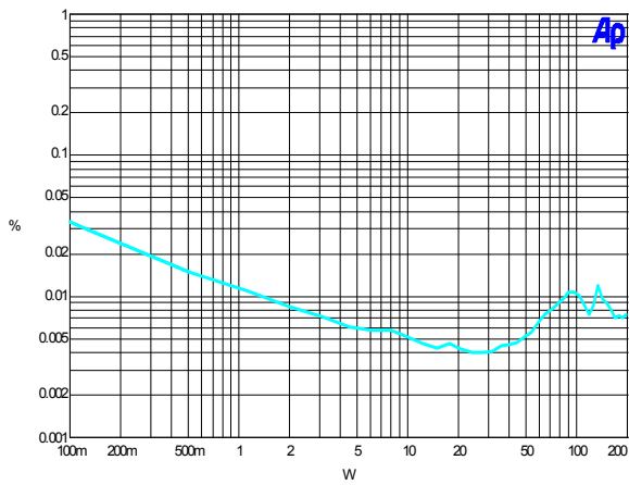
TIM vs. output power. R L = 4Ω.
