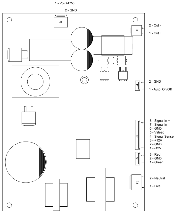
Figure 2: ICEpower200ASC connections
