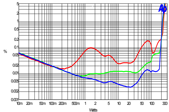
THD+N vs. Po at 100Hz, 1kHz and 6.67kHz 8) (4Ω), 110Vac/60Hz
