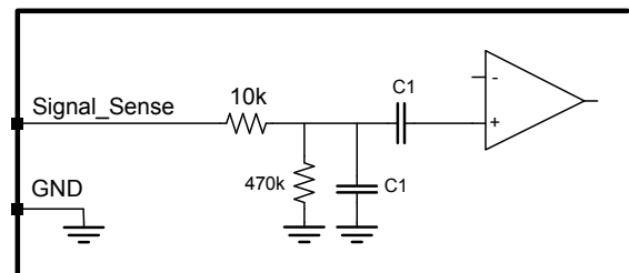
Figure 13: Signal_Sense input
