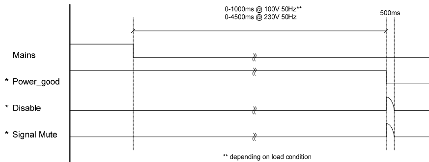
Figure 21: Power down after mains off. * denotes an internal signal.
