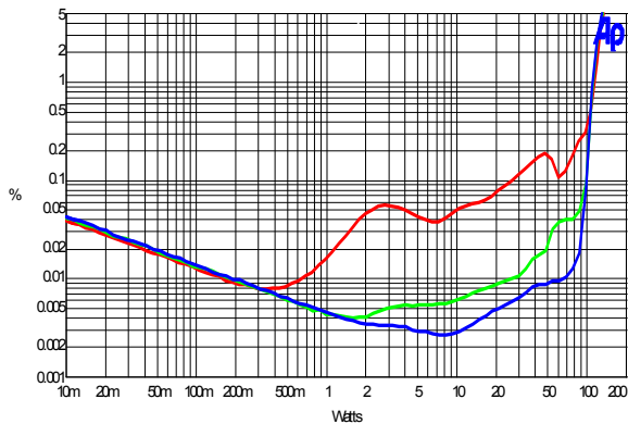
THD+N vs. Po at 100Hz, 1kHz and 6.67kHz 8) (8Ω), 110Vac/50Hz
