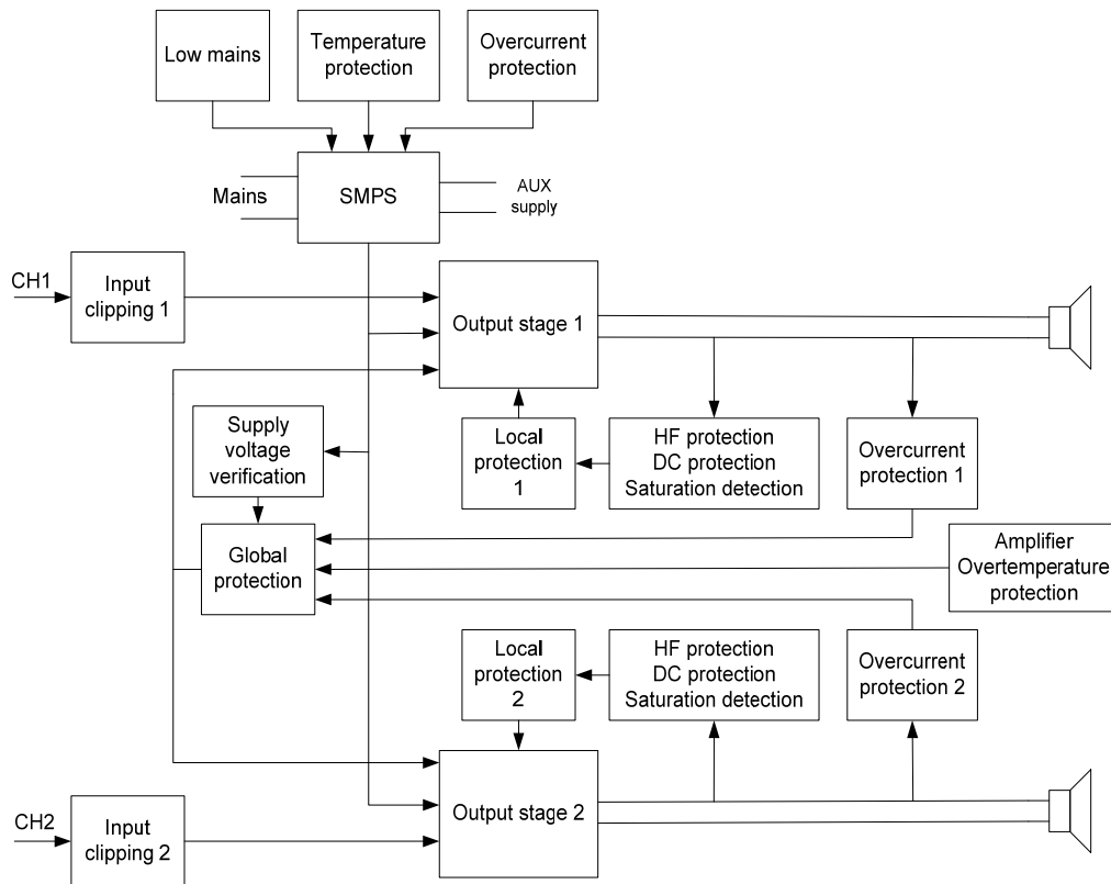
Figure 15: Protection schematic
