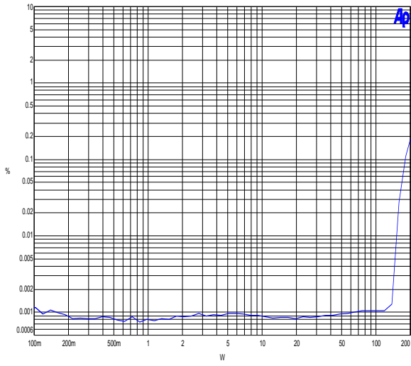
CCIF IMD vs. P_0 , R_L = 4\Omega , f_1 = 18.5\text{kHz} , f_2 = 1\text{kHz} , IMD@10W = 0.0009%.
