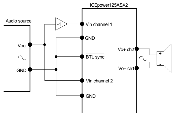
Figure 17: Wiring diagram for the BTL module
