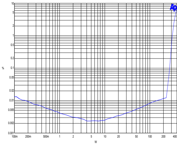
TIM vs. output power. R_L = 4\Omega , TIM@10W = 0.003%
