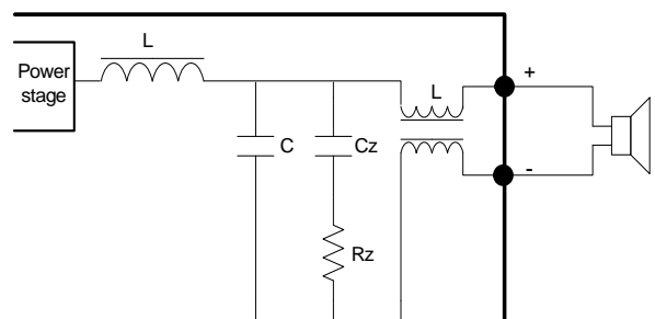
Figure 18: SE output filter section with compensating Zobel network
