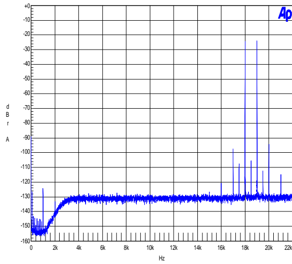
CCIF IMD analysis. R_L = 4\Omega , P_0 = 10\text{W} .
