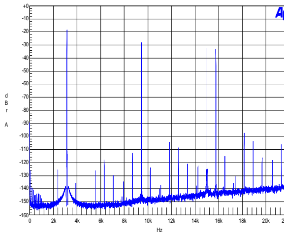
TIM FFT analysis. R_L = 4\Omega , P_0 = 10\text{W} .
